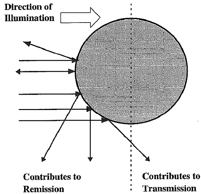
Fig. 5. Illustration of the fact that regular reflection from the external surface of a particle contributes to transmission as well as remission.
